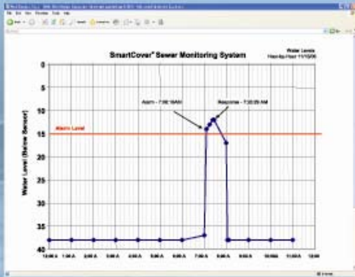
Detail of surcharge alarm showing results of early response. A sewage spill was prevented.
